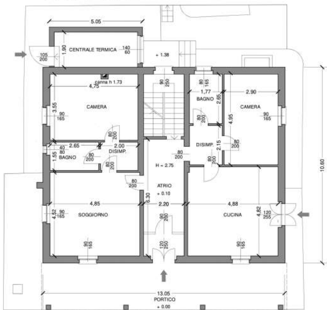
PIANO TERRA
