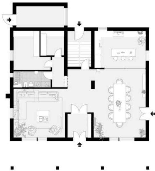
PIANO TERRA
